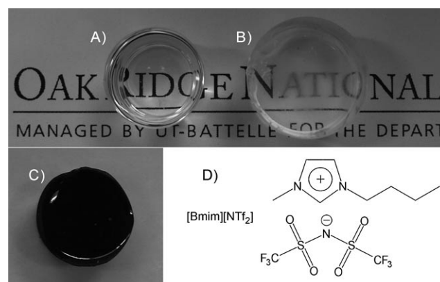
Figure 1. Transparent monolithic silica gels containing different amounts of [Bmim][NTf 2 ] ( x=0.3 and 2.0 for (A) and (B), respectively). After heat treatment under N 2 , the clear monolith (A) turned black (C). D) Structure of [Bmim][NTf 2 ].
